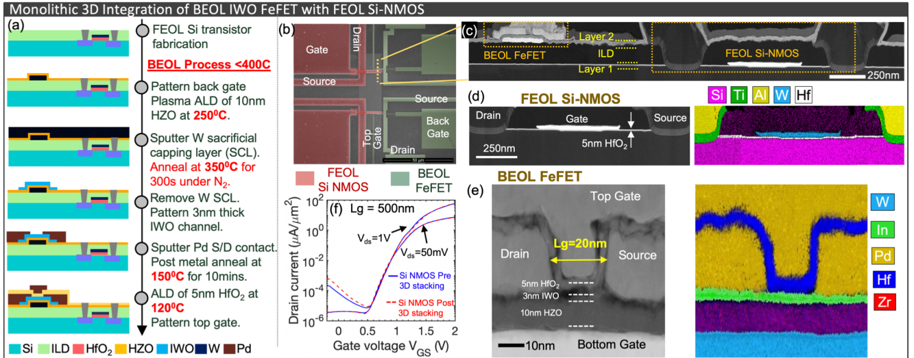
Fig. 2(a) Key fabrication steps in M3D integration of BEOL FeFET on top of FEOL Si-NMOS highlighting low thermal budget. (b) Tow view false-colored SEM of the M3D integrated structure. (c) STEM showing cross-section of fully processed 2-tier M3D integrated structure with BEOL FeFET (top device layer) and FEOL Si-NMOS (bottom device layer). (d, e) STEM and EDS elemental map of 500nm L G FEOL Si-NMOS and 20nm L G BEOL FeFET, respectively. (f) Measured I D -V G of FEOL Si-NMOS pre and post 3D stacking showing matched transfer characteristics. The post 3D stacking Si-NMOS characteristics was measured after subjecting to full BEOL processing of FeFET.
