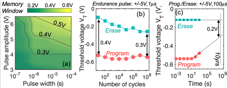
Fig. 7(a) Dependence of MW on program pulse amplitude and pulse width highlighting the switching speed of FeFET. Write operation with \pm 5\text{V} , 1\mu\text{s} is achieved. (b) High endurance >10^8 cycles and (c) high retention with no degradation in memory window measured in IWO FeFET at 25^\circ\text{C} .
