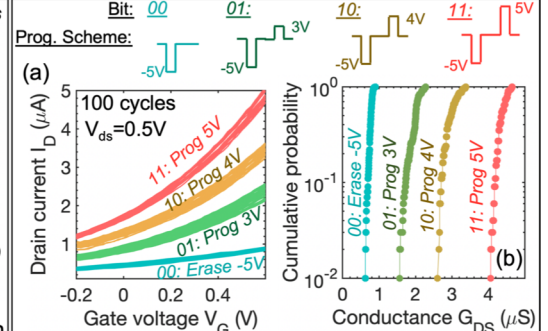
Fig. 8(a) Demonstration of multi-bit program capability of IWO FeFET. 4 tightly distributed distinct I_D levels achieved using different programming schemes. (b) Distribution of well separated 4 conductances measured for 100 cycles.
