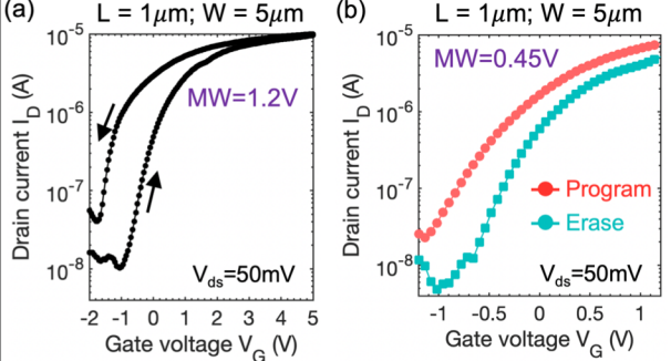
Fig. 5(a) Measured pulsed I_D - V_G of FeFET for -2\text{V} to +5\text{V} V_G sweep showing large MW of 1.2V. (b) Measured I_D - V_G using a single program and erase pulse of \pm 5\text{V} , 100\mu\text{s} showing 0.45V MW.
