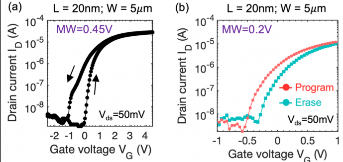
Fig. 6(a) Measured pulsed I_D - V_G of ultra-scaled FeFET of L_g=20\text{nm} for -2\text{V} to +5\text{V} V_G sweep showing MW of 0.45V. (b) Using a single program and erase pulse of \pm 5\text{V} , 100\mu\text{s} , MW of 0.2V was obtained.
